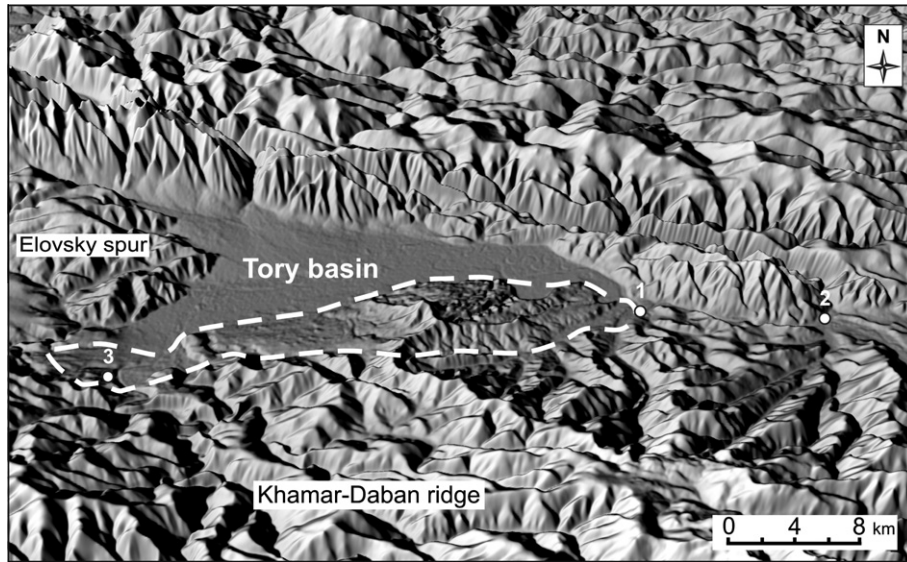
Fig. 9. The eastern part of the Tunka rift basin (based on SRTM digital elevation data). Dashed line indicates the area of inversion (uplifted part of the Tory basin). Numbers correspond to sections: 1 – Tibelti; 2 – Anchuk; 3 – Slavin Yar.
